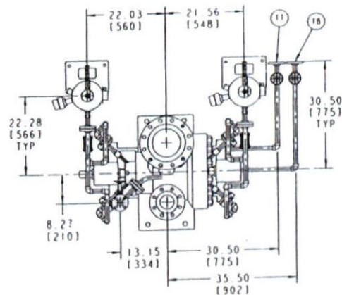
PLAN 52 PARTS LIST - STAINLESS 3/4" SOCKET WELDED PIPE EXTERNAL FLUID RESERVOIR, NONPRESSURIZED, WITH FORCED CIRCULATION, AS REQUIRED
