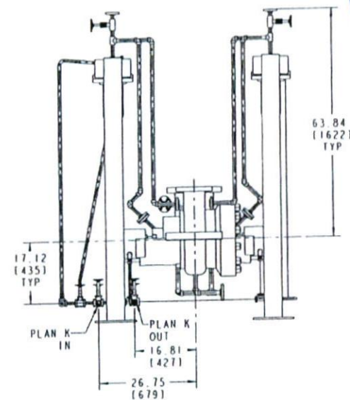
PLAN 21 PARTS LIST - 316SS 1/2" SOCKET WELDED PIPE (CIRCULATION FROM PUMP DISCHARGE THRU COOLER AND BACK TO THE SEAL CHAMBER)
